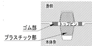
[A矢視図]
